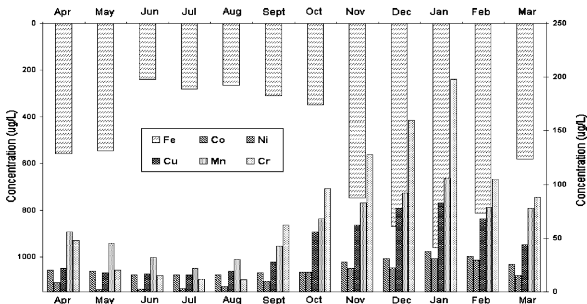
Figure 2 Seasonal variation of metal ions.
