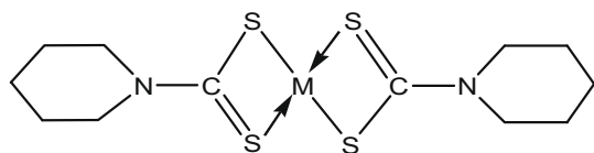
Figure 1 Structural diagram of PMDTC–metal complex.
